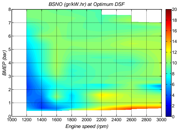
Figure 17: BSNO map of engine with V8 and DSF operations
