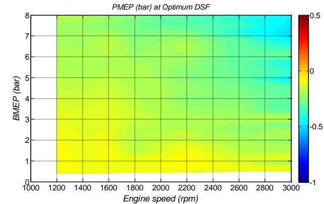
Figure 4: The contour plots of pumping loss for V8 and DSF operations as a function of BMEP and engine rpm (test matrix shown in Table 2)
