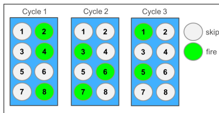
Figure 1: DSF operation of 1 fire - 2 skips for each cylinder in an eight cylinder engine
